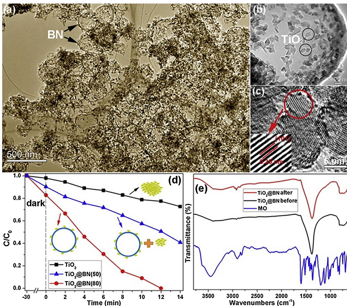
Fig. 6. (a, b) TEM images of TiO 2 @BN(80) hollow nanospheres hybrid. (c) HRTEM image of TiO 2 NCs. Inset shows the magnified interplanar spaces of TiO 2 labeled. (d) Photocatalytic degradation curves of MO with BN, TiO 2 NCs, TiO 2 @BN(50), and TiO 2 @BN(80). (e) FTIR spectra of MO, TiO 2 @BN hybrids before and after reaction. Reproduced with permission from Ref. [109]. Copyright 2017, ACS.
