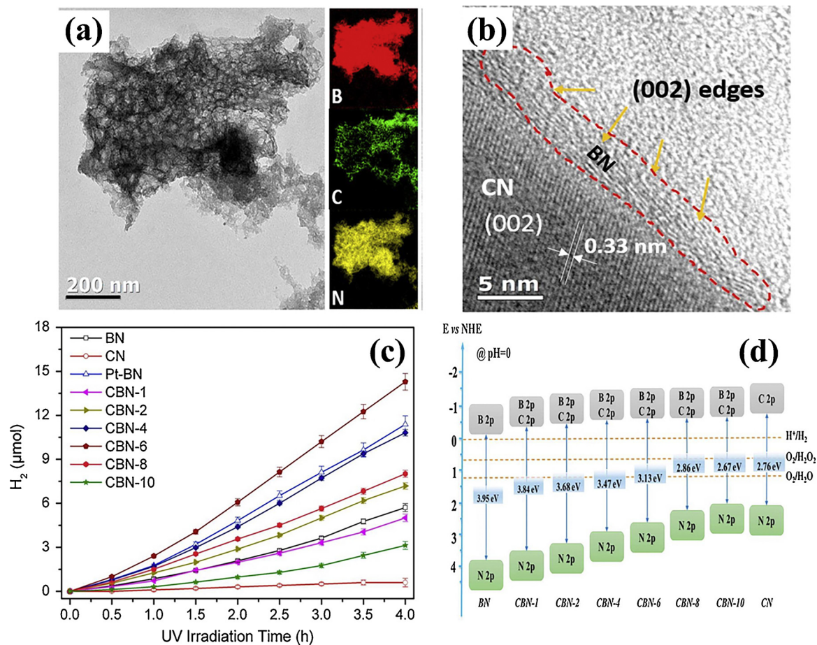
Fig. 10. (a–b) TEM images and EELS mapping data of CBN-6, (c) Time profiles of photocatalytic H 2 production in the presence of BN, CN or CBN- x samples. (d) Determined band energy levels of CBN- x electrodes, in comparison with pure h -BN and CN electrodes. The standard reduction potentials for H + /H 2 , O 2 /H 2 O 2 and O 2 /H 2 O couples are shown as a reference. Reproduced with permission from Ref. [57]. Copyright 2017, Elsevier.
