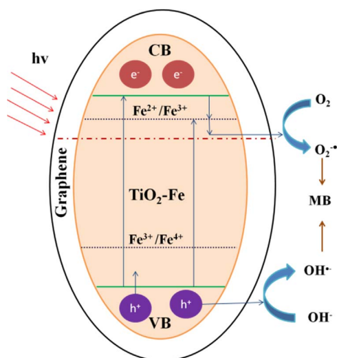
Fig. 8. Proposed mechanism for the enhanced visible light photocatalytic activity of G- TiO_2 -Fe.
