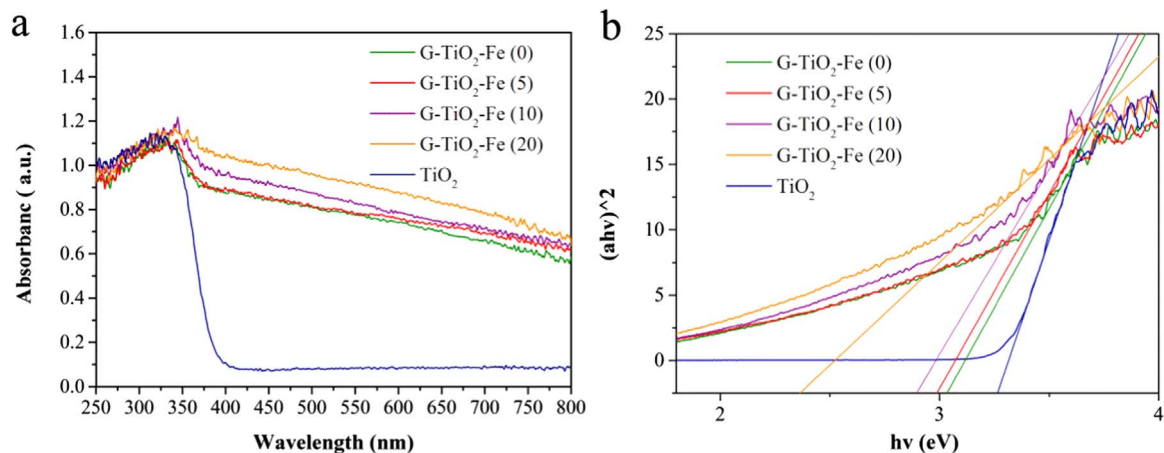
Fig. 6. Diffuse reflectance spectra (a) and plots of the Kubelka-Munk remission function (b) for TiO 2 NP, G-TiO 2 -Fe (5), G-TiO 2 -Fe (10) and G-TiO 2 -Fe (20).
