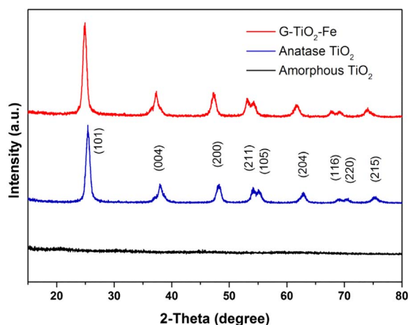
Fig. 2. X-ray diffraction patterns of amorphous TiO 2 , anatase TiO 2 and G-TiO 2 -Fe.
