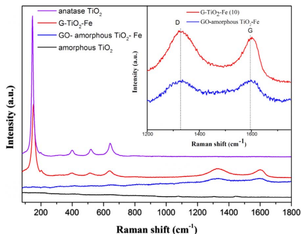
Fig. 3. Raman spectra of bare amorphous \text{TiO}_2 NPs, anatase \text{TiO}_2 , GO-amorphous \text{TiO}_2\text{-Fe} and G- \text{TiO}_2\text{-Fe} .
