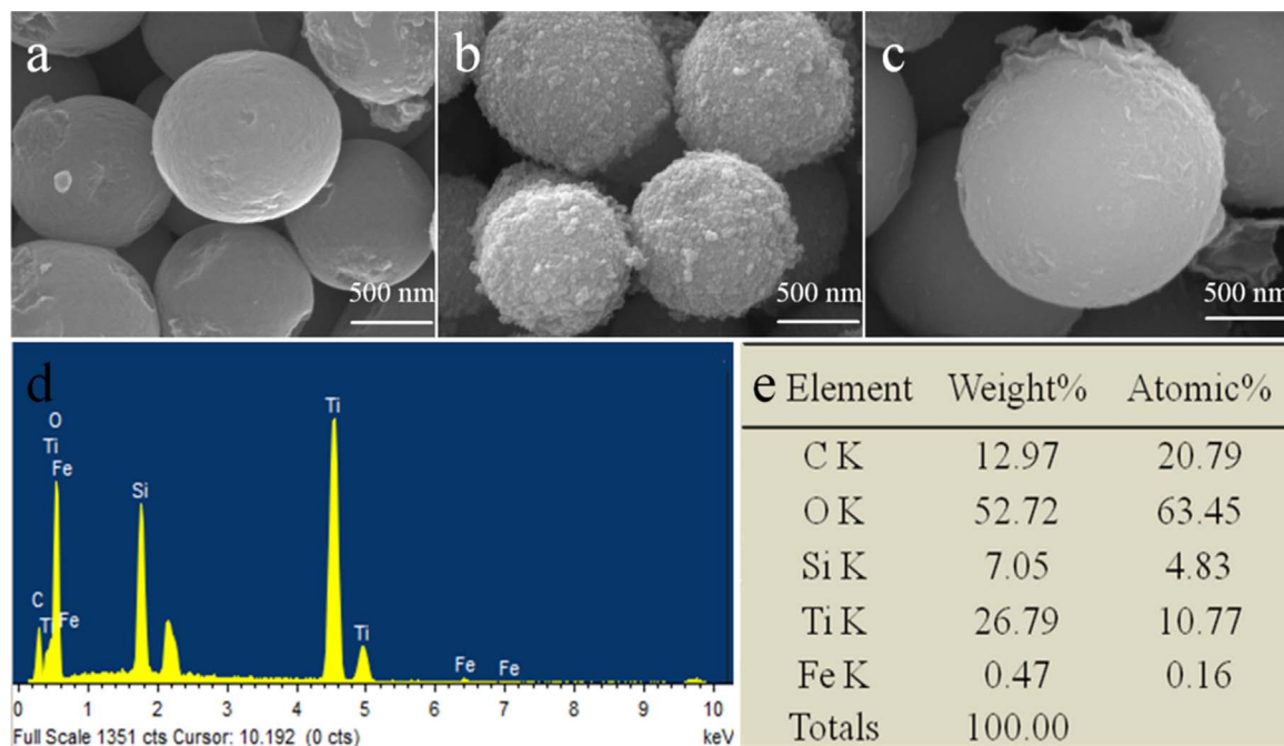
Fig. 4. FE-SEM images of amorphous \text{TiO}_2 (a), anatase \text{TiO}_2 (b) and G- \text{TiO}_2\text{-Fe} (10) (c) and EDS analysis results (d, e) of G- \text{TiO}_2\text{-Fe} (10).
