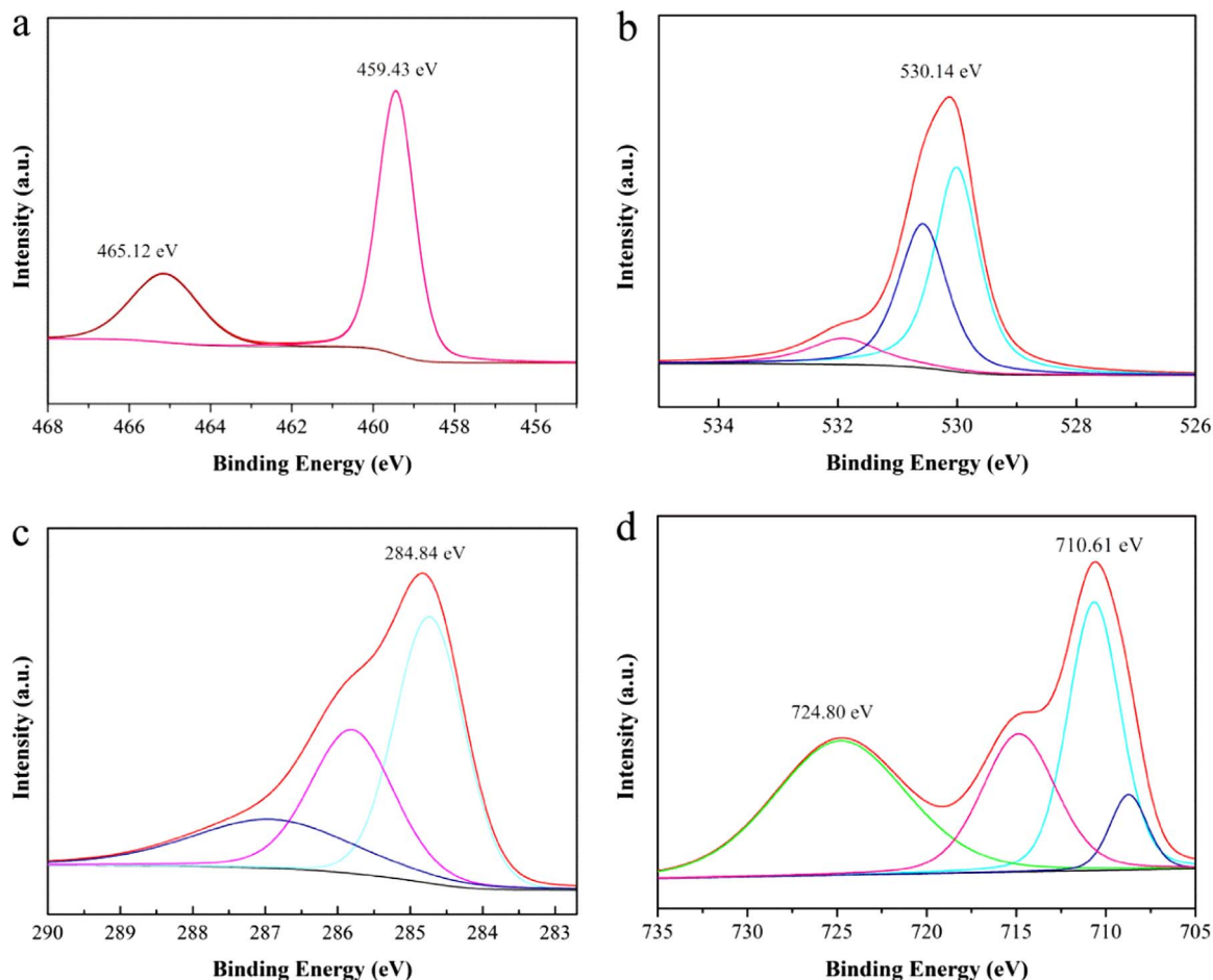
Fig. 5. XPS core level spectra of Ti 2p (a), O 1s (b), C 1s (c), and Fe 2p (d) of G-TiO 2 -Fe (10) sample.
