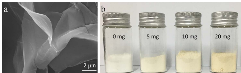
Fig. 1. FE-SEM image of GO sheets (a) and the amorphous TiO 2 with different Fe doping amounts (b).
