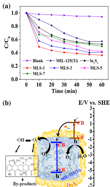
Fig. 9. (a) Photocatalytic performance of \text{In}_2\text{S}_3 , MIL-125(Ti) and MLS for TC degradation. (Experimental conditions: initial TC concentration = 46 mg/L, pH 5.9, m = 30 mg, V = 100 mL) For comparison, photocatalytic performance for no photocatalyst is also given. (b) Schematic illustration of photo-generated charge carrier's separation and transfer in core-shell MLS sample.
