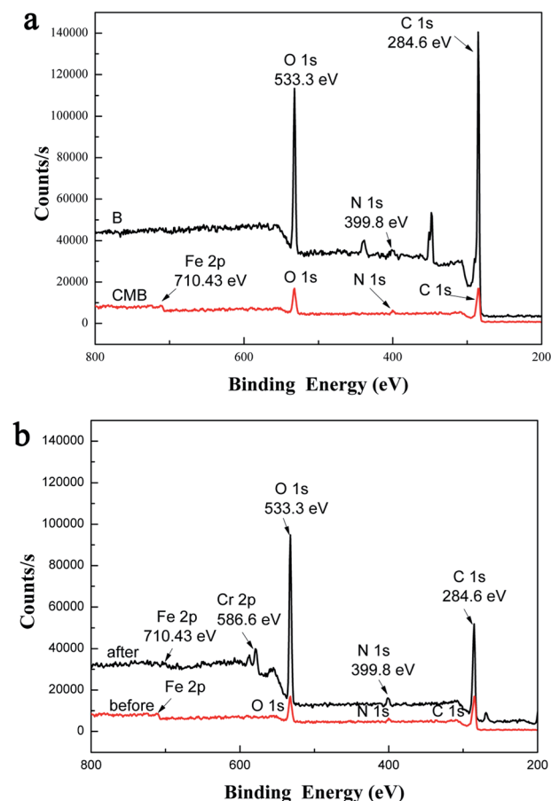
Fig. 4 (a) XPS survey spectra of B and CMB, (b) XPS survey spectra of CMB before and after adsorption.
