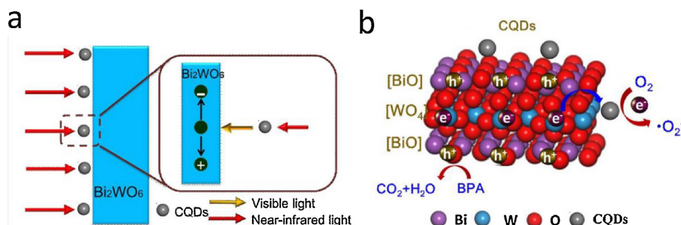
Fig. 9. (a) Schematic diagram for up converted PL of OD CQDs modified 2D ultrathin BWO nanosheets heterojunctions; (b) proposed photocatalytic mechanism of CBW under full spectrum light irradiation. Reprinted from Ref. [139] with permission from Elsevier.
