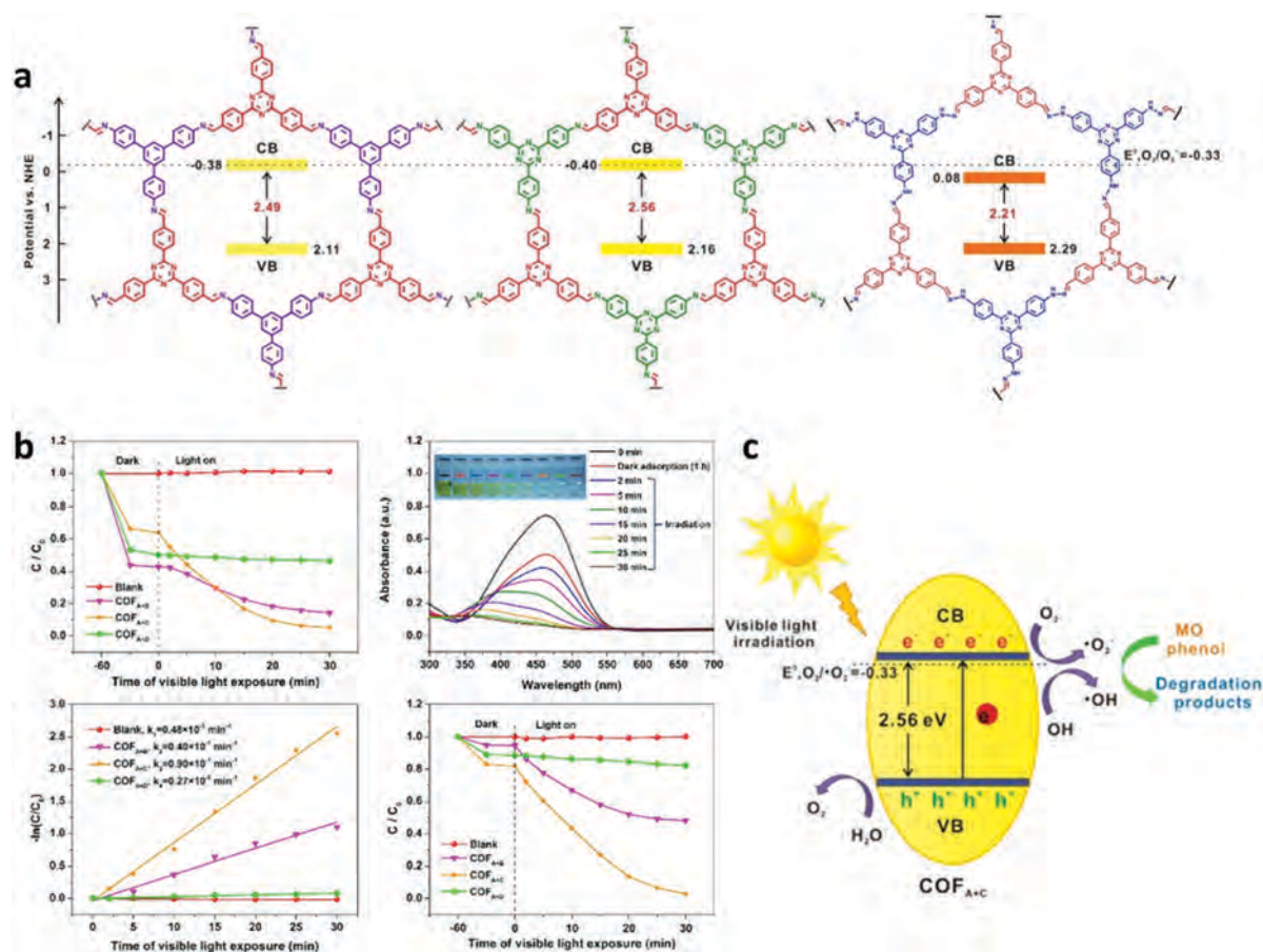
Fig. 15 (a) Structure and band alignment of COF A+B , COF A+C and COF A+D . (b) Photocatalytic performance of COF A+B , COF A+C and COF A+D under visible light irradiation. (c) Schematic illustration of pollutant photodegradation over COF A+C under visible light irradiation. Reproduced with permission from ref. 253. Copyright 2017, Elsevier B. V.
