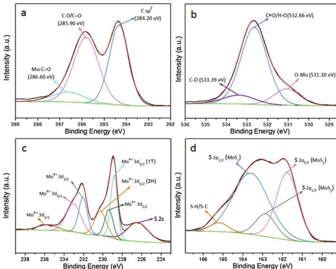
Fig. 3. High resolution XPS spectrum of C 1s (a), O 1s (b); Mo 3d (c); and S 2p (d) in g\text{-MoS}_2/\text{PGBC} .
