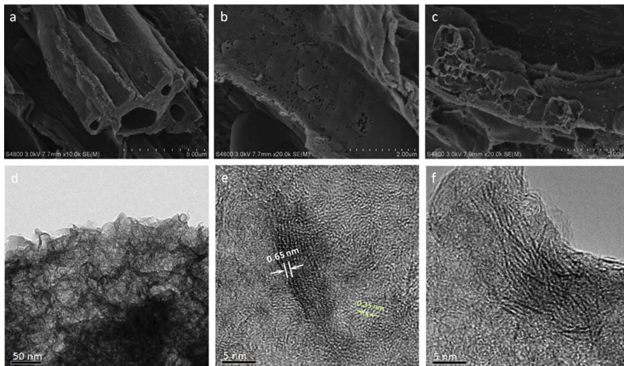
Fig. 1. SEM images of pristine porous graphitic carbon biochar (a and b) and g\text{-MoS}_2/\text{PGBC} (c), TEM image of g\text{-MoS}_2/\text{PGBC} (d), and HRTEM images of g\text{-MoS}_2/\text{PGBC} (e and f).
