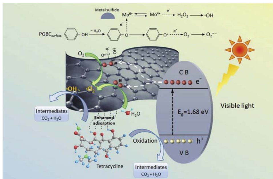
Fig. 8. Schematic illustration of the proposed mechanism for the degradation behavior of TC molecules by g -MoS 2 /PGBC nanocomposite under visible light irradiation.
