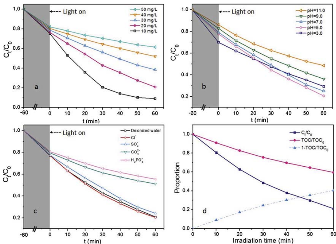
Fig. 6. Effect of initial TC concentrations (a); initial pH (b), and coexisting anions (c) on the degradation of TC over g -MoS 2 /PGBC; the photodegradation and TOC removal curves (d) of TC on g -MoS 2 /PGBC under visible light irradiation.
