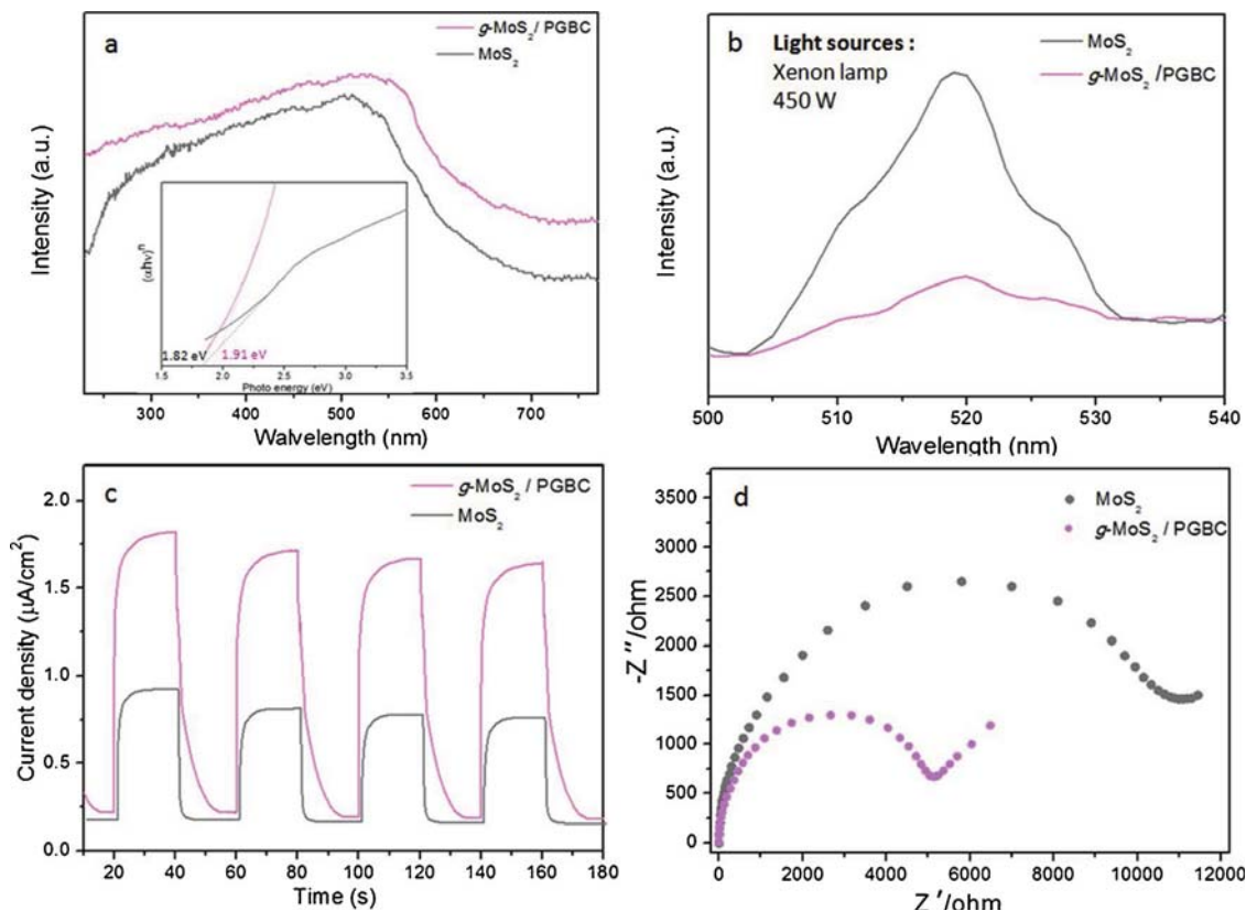
Fig. 4. UV–vis diffuse reflectance spectra and the plots of (\alpha h\nu)^n vs photon energy (h\nu) of as-prepared MoS 2 and g-MoS 2 /PGBC (a); Photoluminescence (PL) spectra (b); transient photocurrent response (c); and electrochemical impedance spectra (d) for the as-prepared samples.
