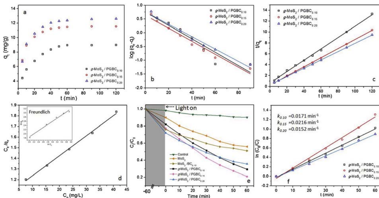
Fig. 5. Effect of contact time on the adsorption of TC onto g -MoS 2 /PGBC under darkness (a); the pseudo-first-order plots (b); pseudo-second-order plots (c); detail equilibrium isotherms: (d) Langmuir model and Freundlich model (inset) for TC adsorption by g -MoS 2 /PGBC under darkness; removal of TC in the presence of different photocatalysts with various composition ratios between g -MoS 2 and PGBC under visible light irradiation (e); photocatalytic rate of g -MoS 2 /PGBC under visible light irradiation (f).
