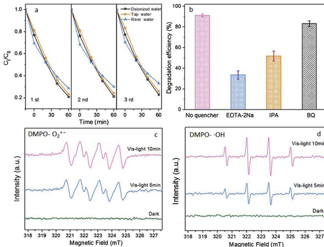
Fig. 7. Cycling performance of photocatalytic degradation for TC removal in different water samples (a); degradation curves of TC with additions of scavengers over g\text{-MoS}_2/\text{PGBC} under visible light (b); and ESR spectra of radical adducts trapped by DMPO in g\text{-MoS}_2/\text{PGBC} dispersion under dark and visible light irradiation: in methanol dispersion for \text{DMPO}\cdot\text{O}_2^- (c); in aqueous dispersion for \text{DMPO}\cdot\text{OH} (d).
