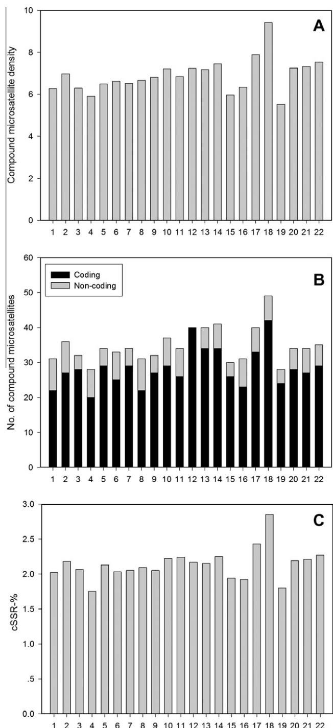
Fig. 1. Distribution of compound microsatellites in analyzed Escherichia coli genomes. (A) Compound microsatellite density (number of compound microsatellites/Mb). (B) Occurrence of compound microsatellites in coding regions and non-coding regions. (C) Percentage of individual microsatellites being part of a compound microsatellite (cSSR-%). x-Axis: S1–S22 complete E. coli genomes.
