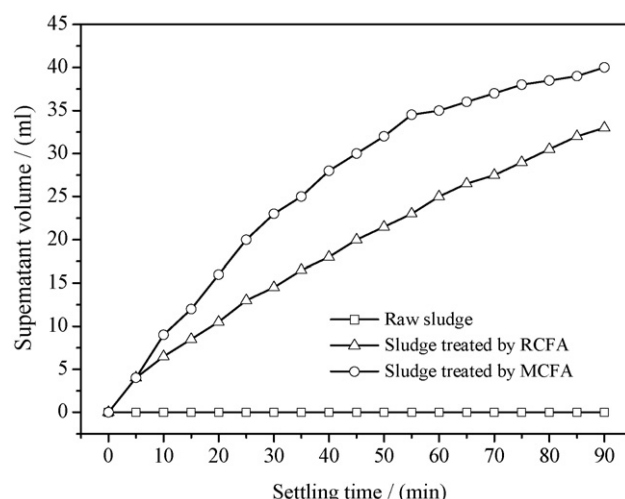
Fig. 5. Settling curve of sludge after conditioning by coal fly ash (coal fly ash dosage, 273%).
