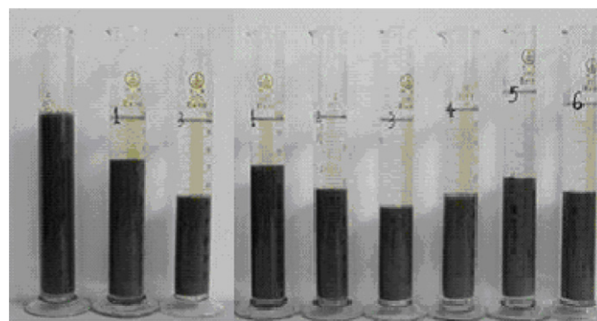
Fig. 6. Sludge settling images of raw sludge, sludge conditioned with RCFA and MCFA (settling time, 60 min). From left to right: 1, raw sludge; 2, sludge conditioned with a RCFA dosage of 273%; 3, sludge conditioned with a MCFA dosage of 273%; 4–9, sludge conditioned with a MCFA dosage of 91%, 273%, 455%, 636%, 818% and 1000%, respectively.
